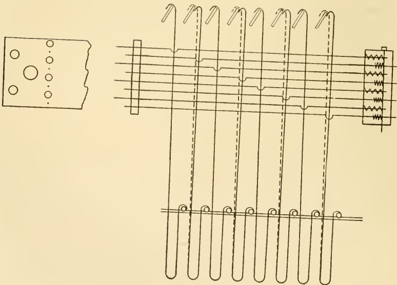
Fig. 8. Hooks Used at the Present Time.
